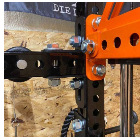
Universal Bracket Connected to Stray Dog Upright
