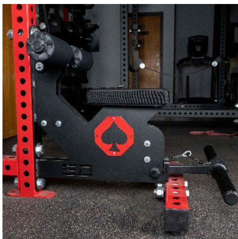
Fixed Lat Seat with logo spot
